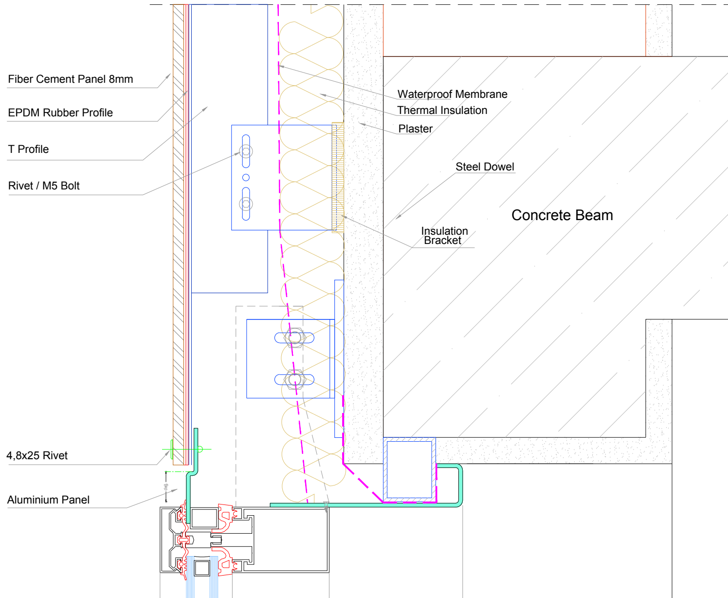
DETAIL B
