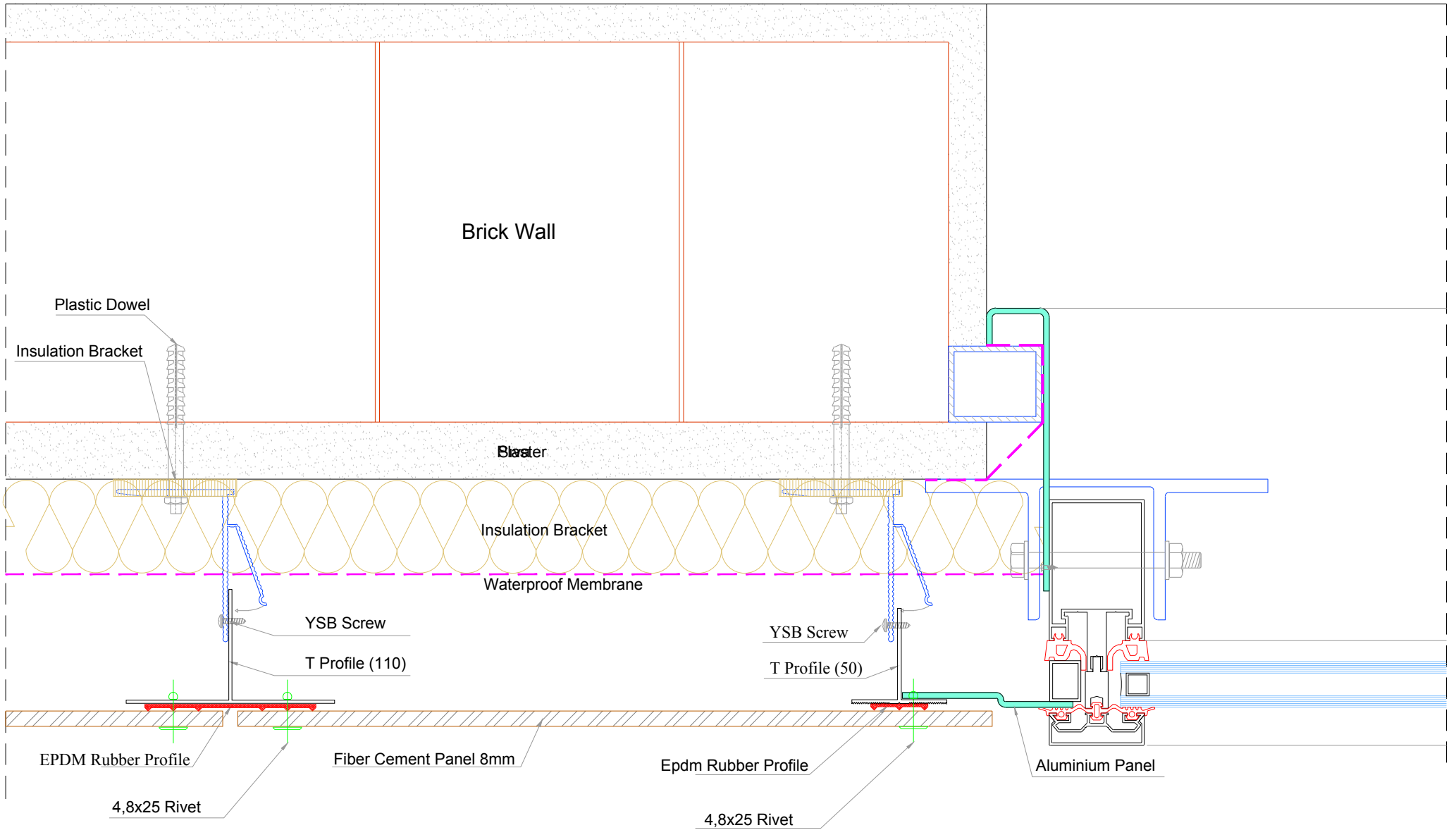
DETAIL A
